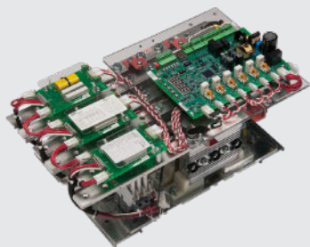
Benshaw RB2 Open Chassis Soft Starter with MX2 Technology
